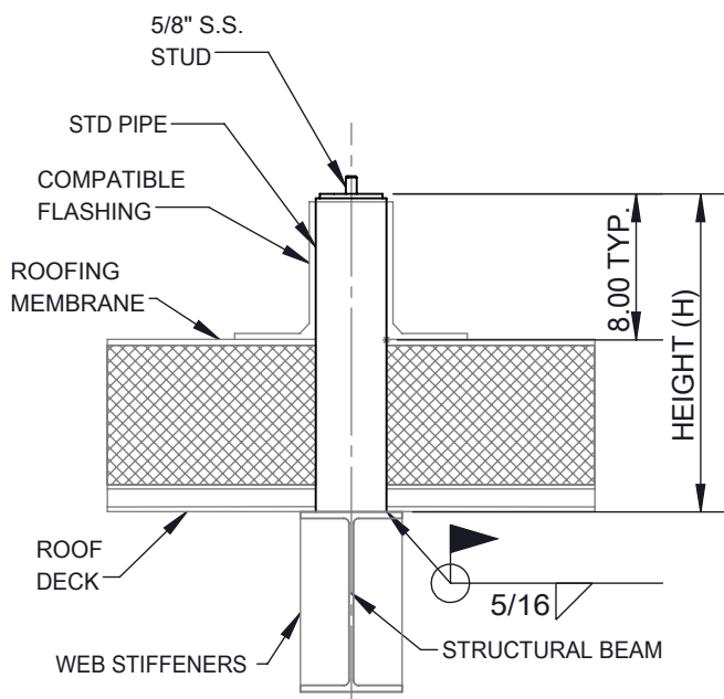
SECTION VIEW - STUD ANCHORAGE
