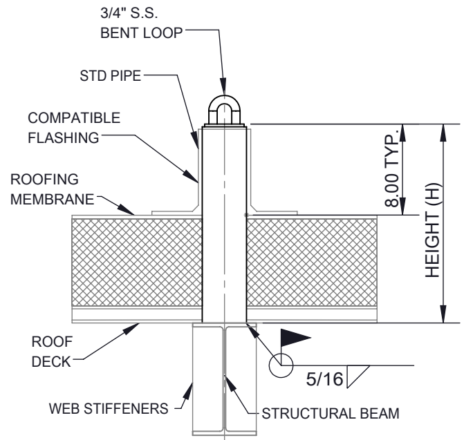
SECTION VIEW - BENT LOOP ANCHORAGE
