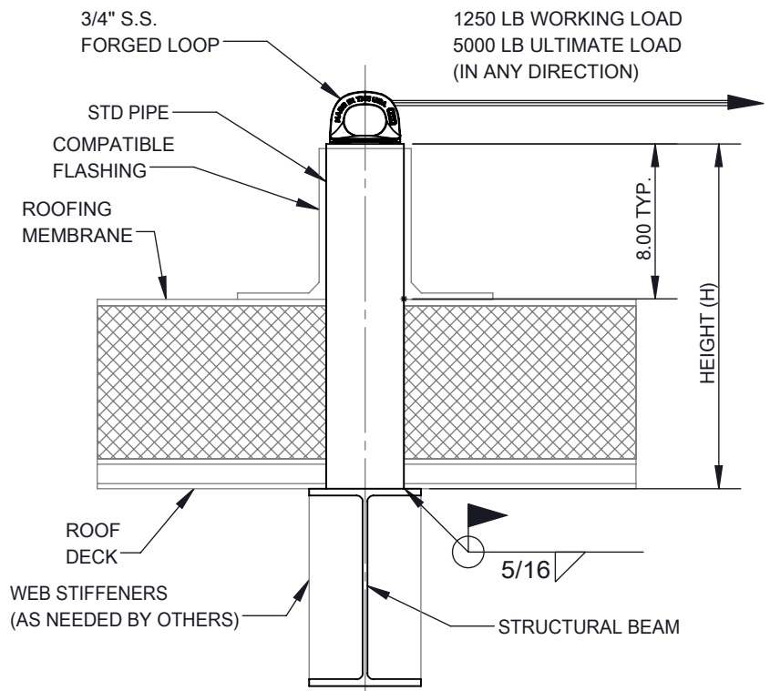
SECTION VIEW - FORGED LOOP ANCHORAGE
