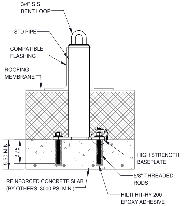
SECTION VIEW - BENT LOOP ANCHORAGE
