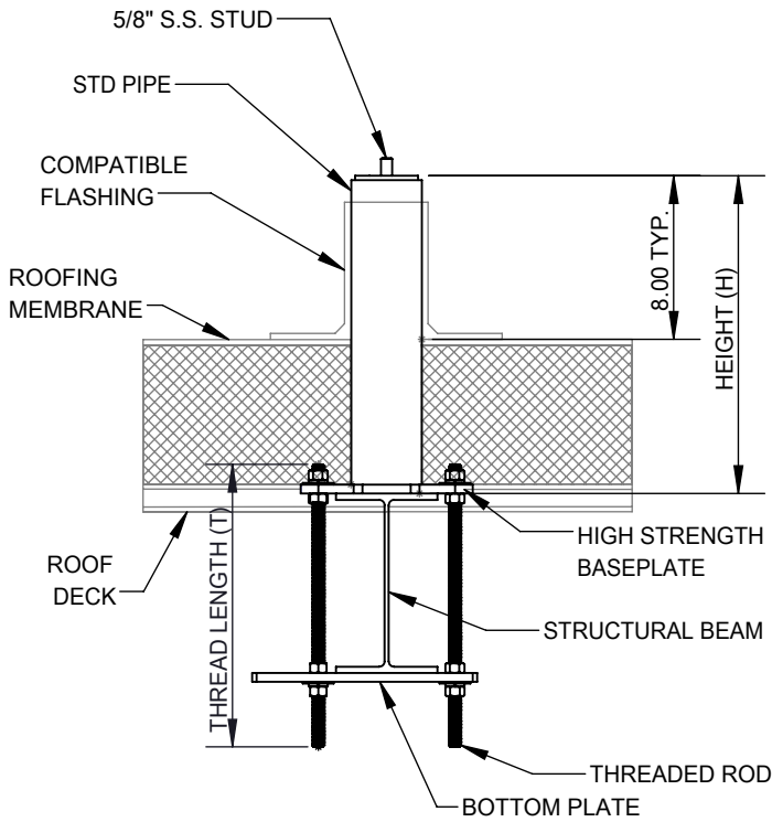
SECTION VIEW - STUD ANCHORAGE
