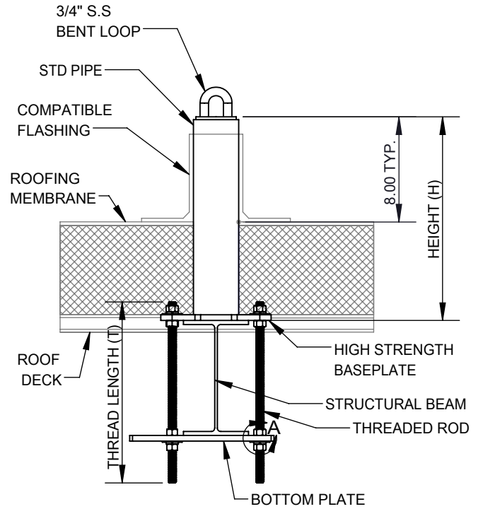
SECTION VIEW - BENT LOOP ANCHORAGE
